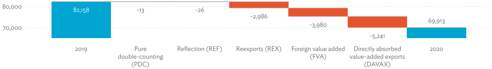
Import Multipliers
