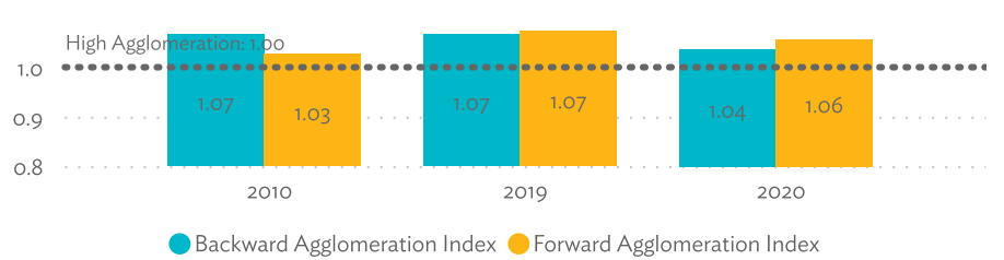
Agglomeration Indices
