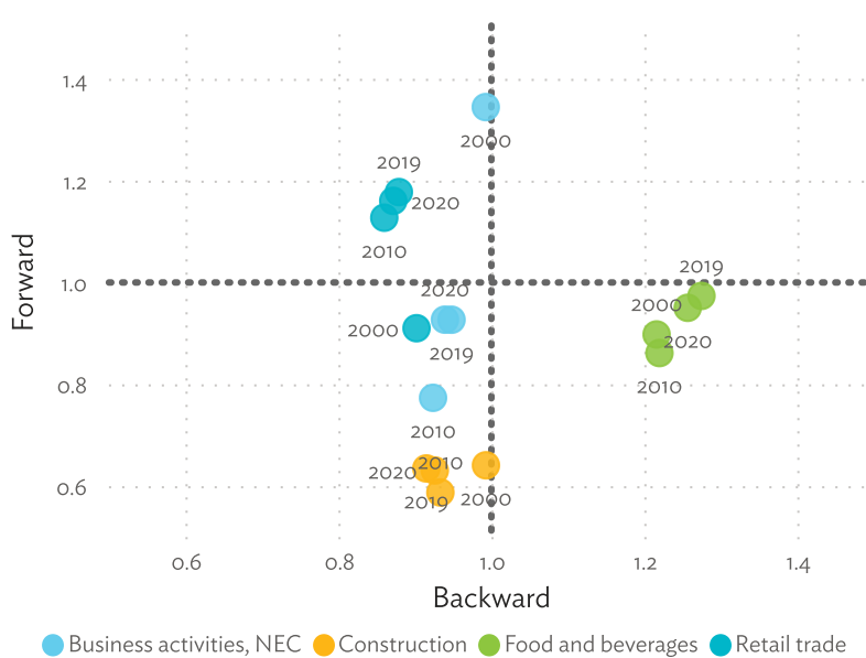
Normalized Linkages
