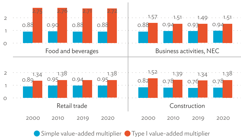
Value-Added Multipliers
